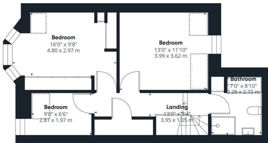
Floor 1
